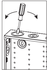
Knockout Removal
